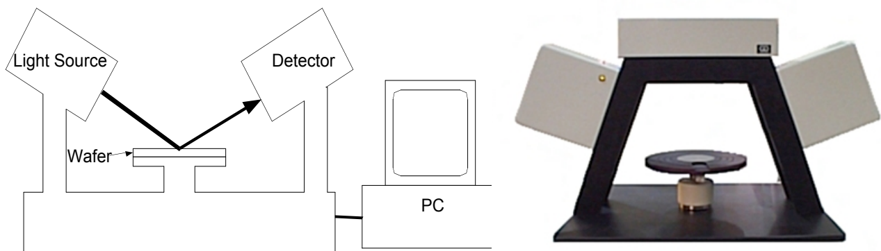
Figure 3: Ellipsometry measurement gauge for film thickness.
